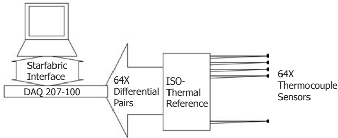
DS 207-250 Sample Application Diagram
