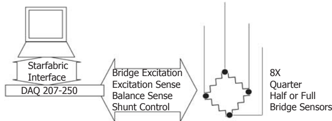
DS 207-250 Sample Application Diagram
