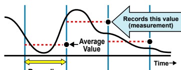
Recording by Average Value Records the average value of the measurements taken every minute within the set recording interval.
