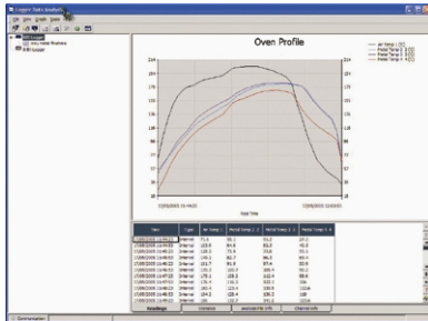
Caption: PaintView Graphical Display for Oven Profile
