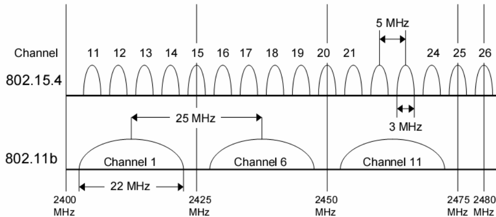
Figure 1: 802.15.4 and 802.11 Frequency Comparisons
