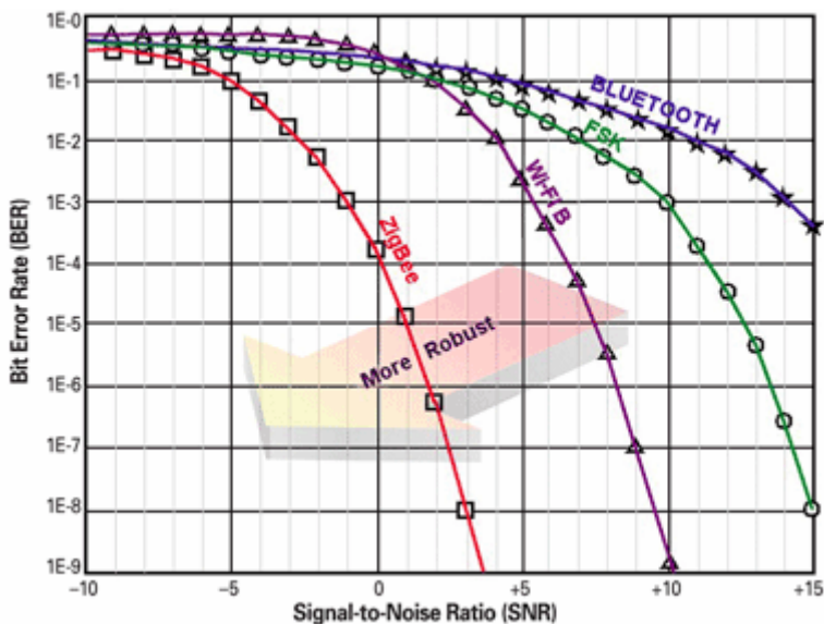
Figure 2: Comparison of modulation techniques at various SNRs
